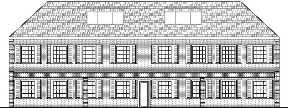
Proposed Rear Elevation Scale 1/6
