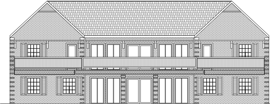
Proposed Front Elevation Scale 1/6
