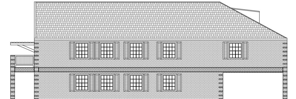
Proposed Right Side Elevation Scale 1/6
